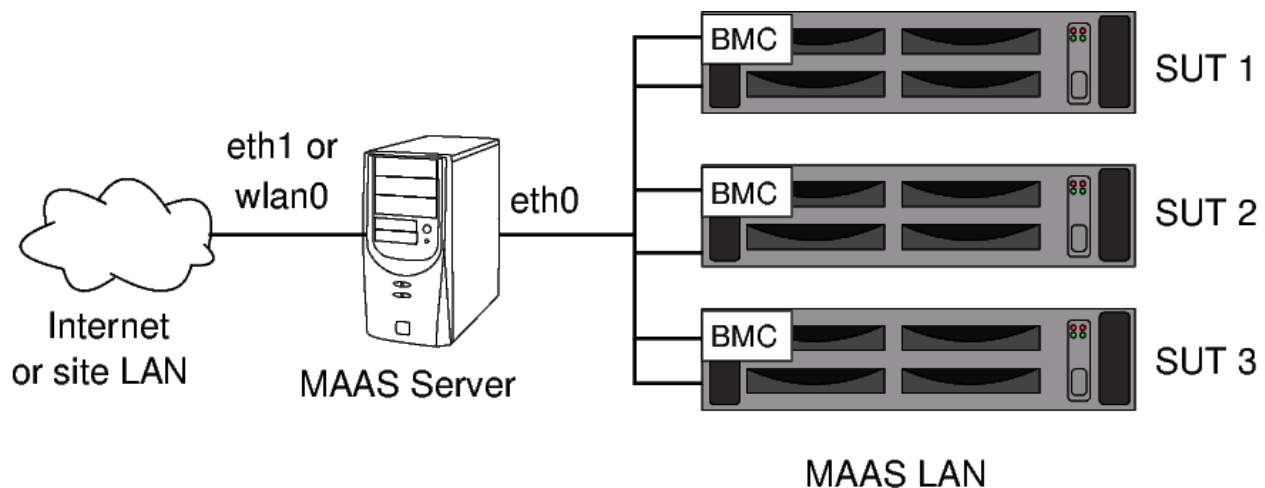
Figure 1: Network structure in which the MAAS server will reside
